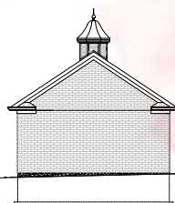
SOUTH ELEVATION
