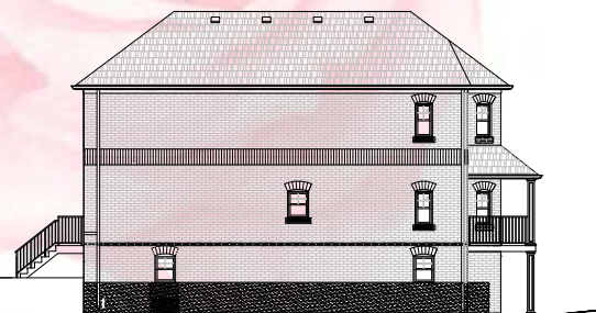
NORTH (BACK) ELEVATION
